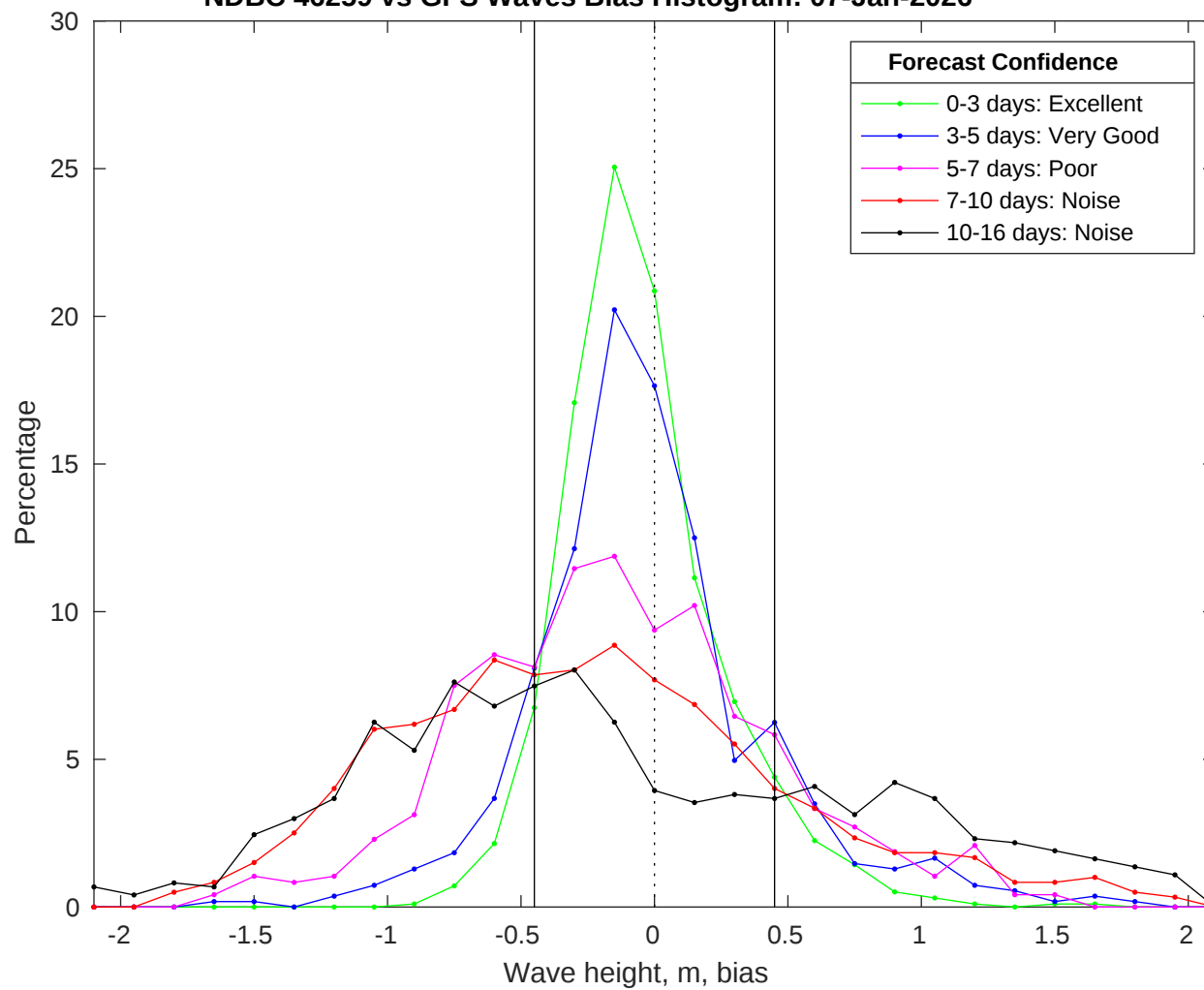
NDBC 46259 vs GFS Waves Bias Histogram: 07-Jan-2026
