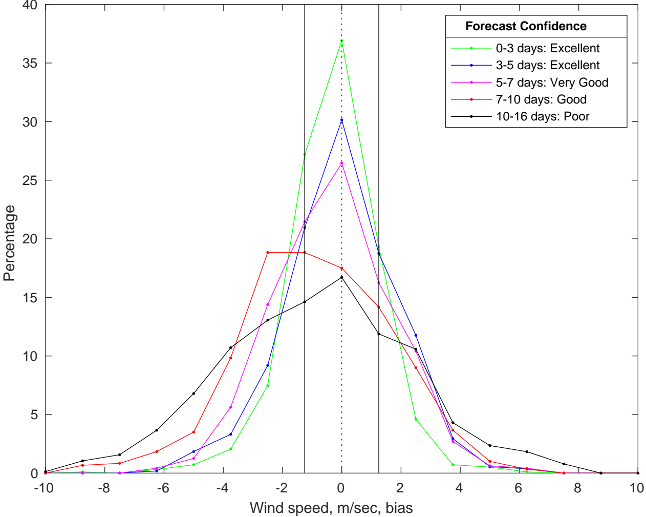
NDBC 51000 vs GFS Winds Bias Histogram: 07-Jan-2026
