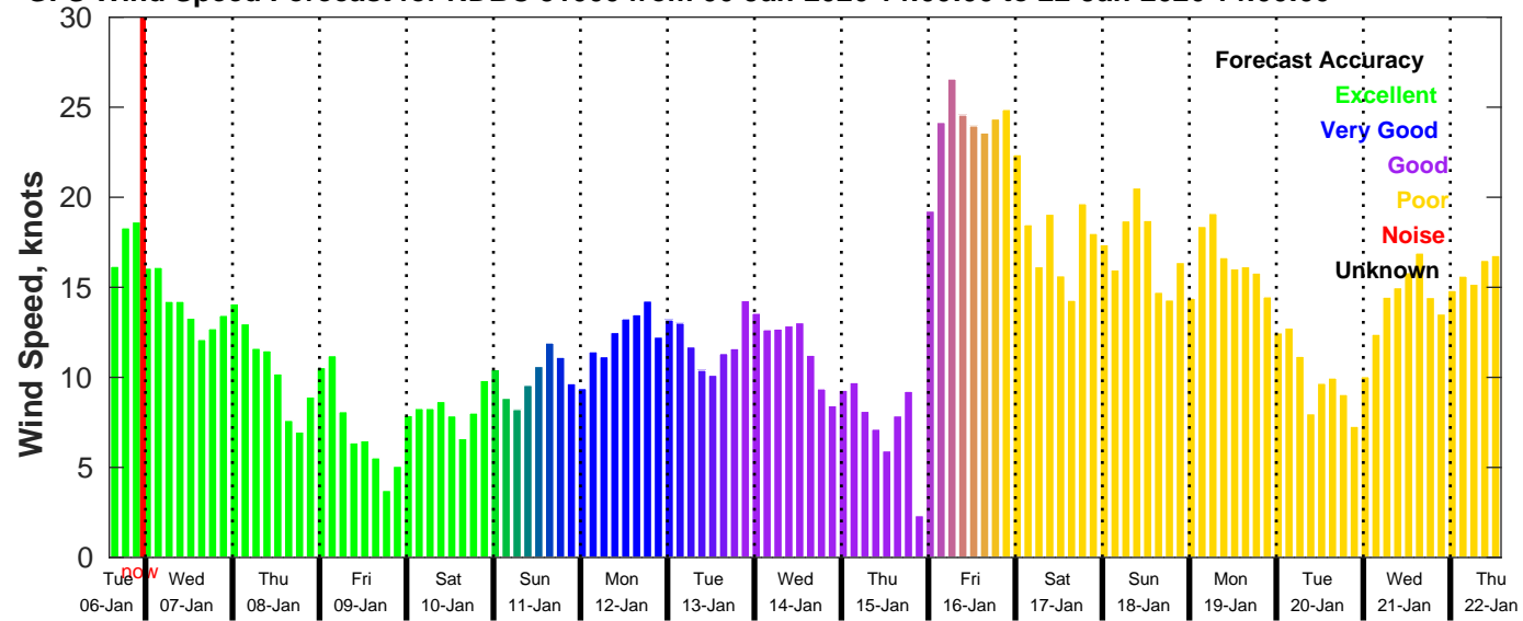
GFS Wind Speed Forecast for NDBC 51000 from 06-Jan-2026 14:00:00 to 22-Jan-2026 14:00:00
