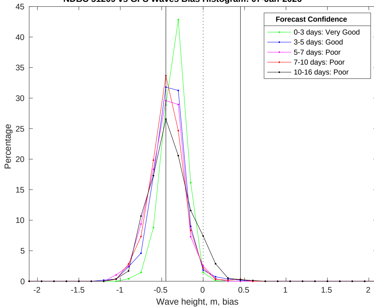
NDBC 51209 vs GFS Waves Bias Histogram: 07-Jan-2026
