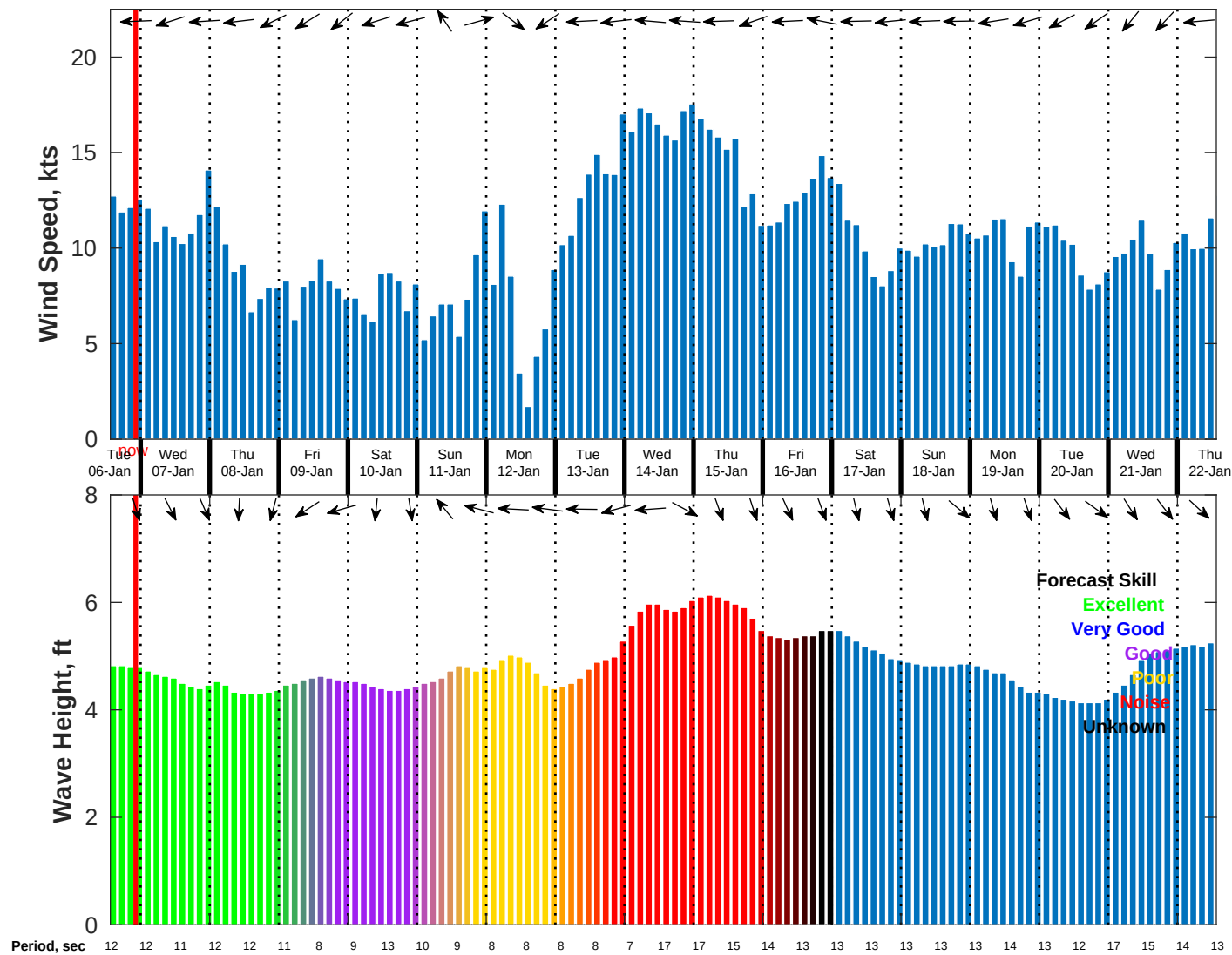
Wind & Wave Forecast for NDBC 51209 from 06-Jan-2026 13:00:00 to 22-Jan-2026 13:00:00
