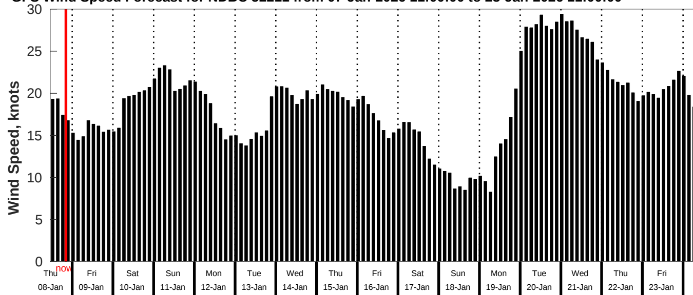
GFS Wind Speed Forecast for NDBC 52211 from 07-Jan-2026 11:00:00 to 23-Jan-2026 11:00:00
