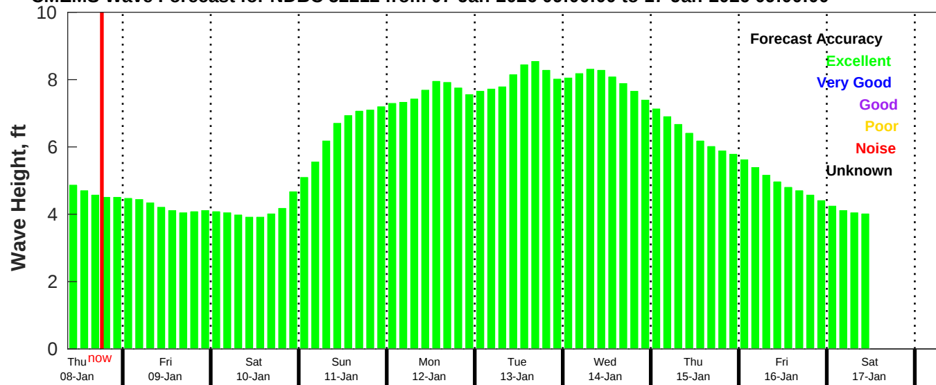
CMEMS Wave Forecast for NDBC 52212 from 07-Jan-2026 09:00:00 to 17-Jan-2026 09:00:00
