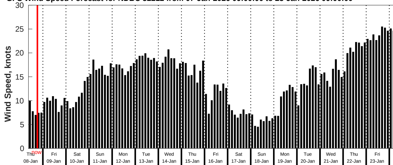
GFS Wind Speed Forecast for NDBC 52212 from 07-Jan-2026 09:00:00 to 23-Jan-2026 09:00:00
