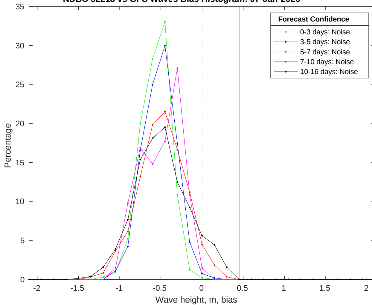
NDBC 52213 vs GFS Waves Bias Histogram: 07-Jan-2026
