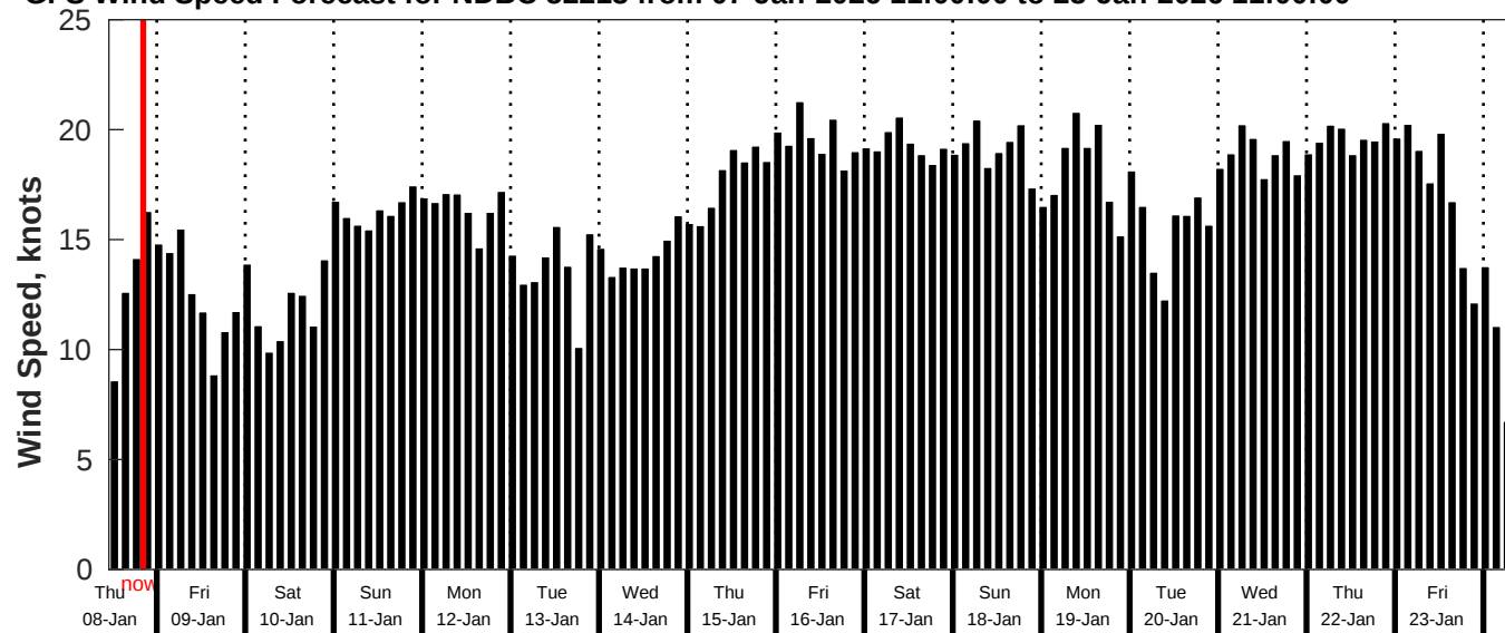
GFS Wind Speed Forecast for NDBC 52213 from 07-Jan-2026 11:00:00 to 23-Jan-2026 11:00:00
