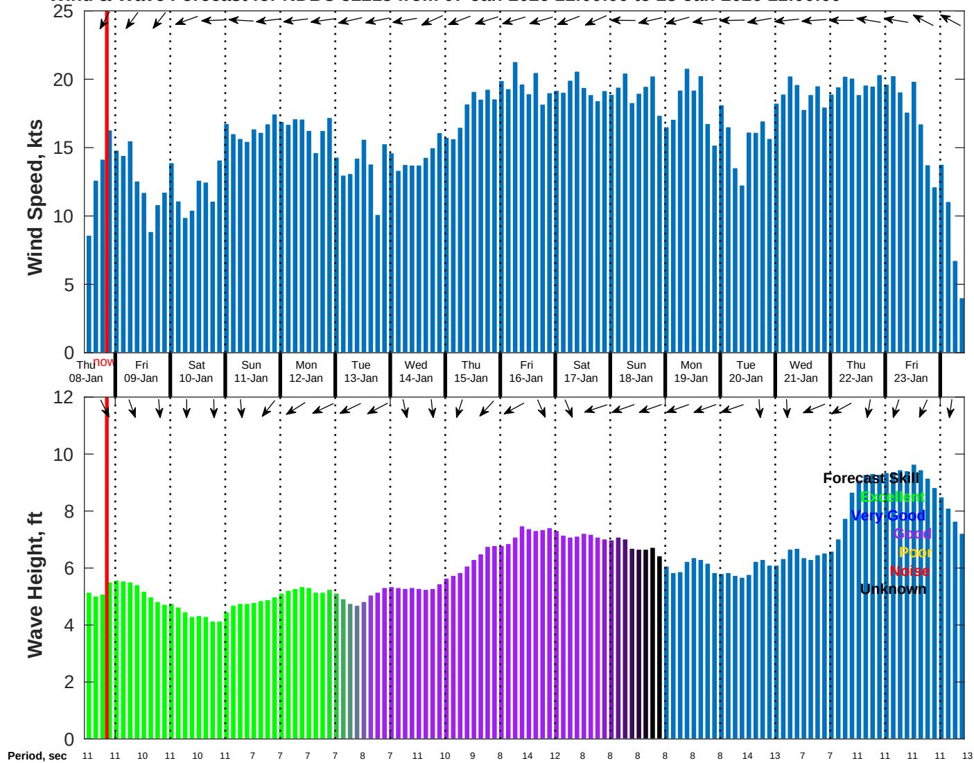
Wind & Wave Forecast for NDBC 52213 from 07-Jan-2026 11:00:00 to 23-Jan-2026 11:00:00
