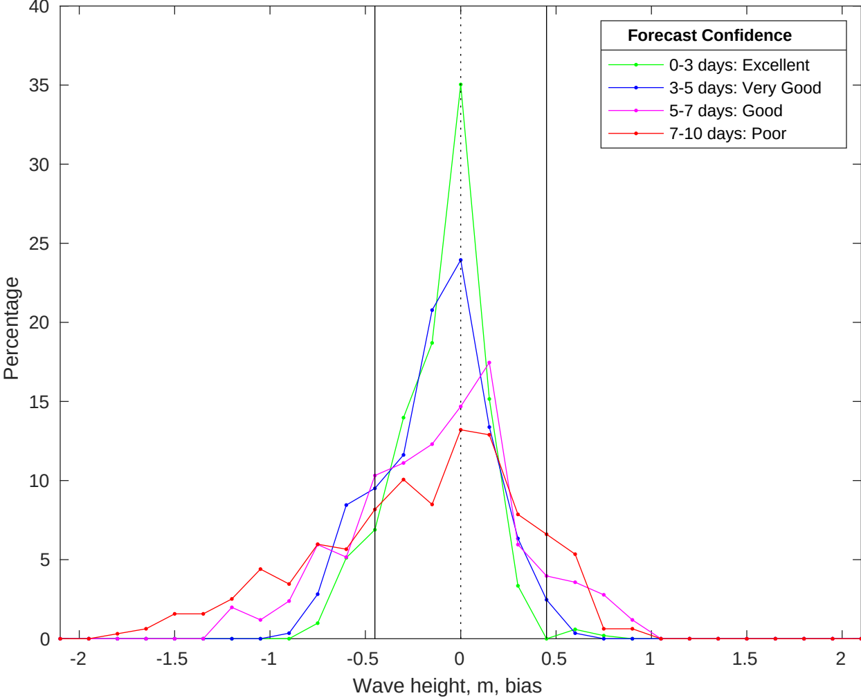
NDBC 41004 vs CMEMS Waves Bias Histogram: 08-Jan-2026
