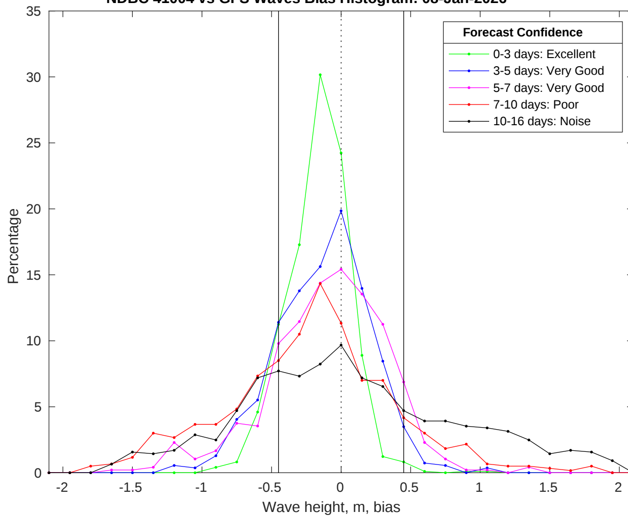
NDBC 41004 vs GFS Waves Bias Histogram: 08-Jan-2026
