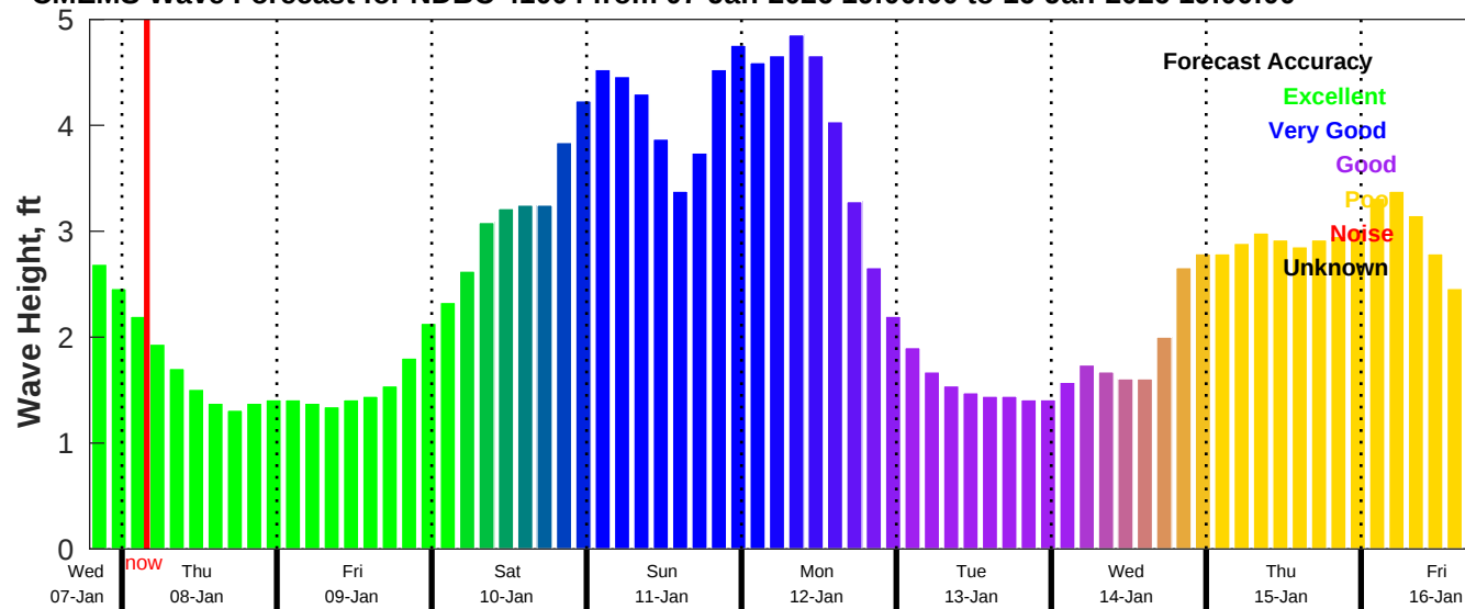
CMEMS Wave Forecast for NDBC 41004 from 07-Jan-2026 19:00:00 to 16-Jan-2026 19:00:00
