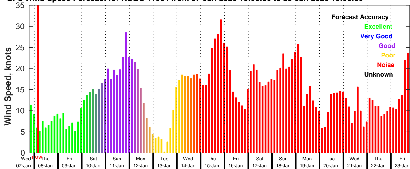
GFS Wind Speed Forecast for NDBC 41004 from 07-Jan-2026 19:00:00 to 23-Jan-2026 19:00:00
