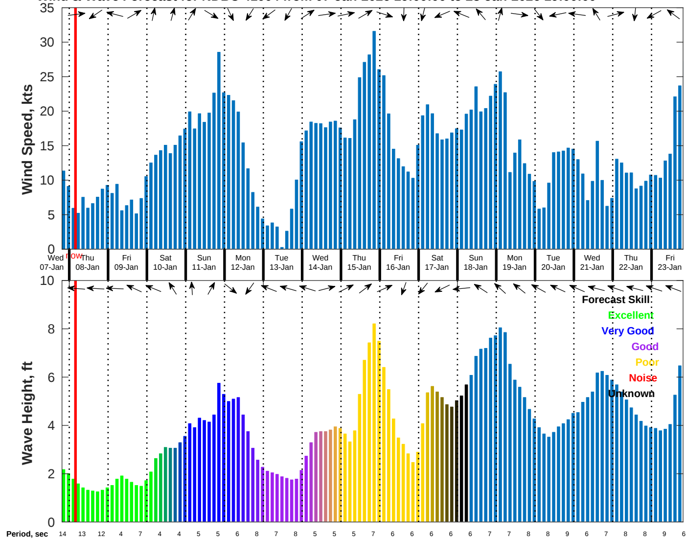
Wind & Wave Forecast for NDBC 41004 from 07-Jan-2026 19:00:00 to 23-Jan-2026 19:00:00
