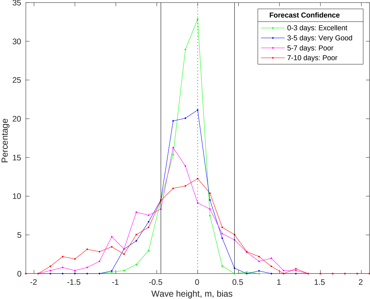
NDBC 41013 vs CMEMS Waves Bias Histogram: 08-Jan-2026
