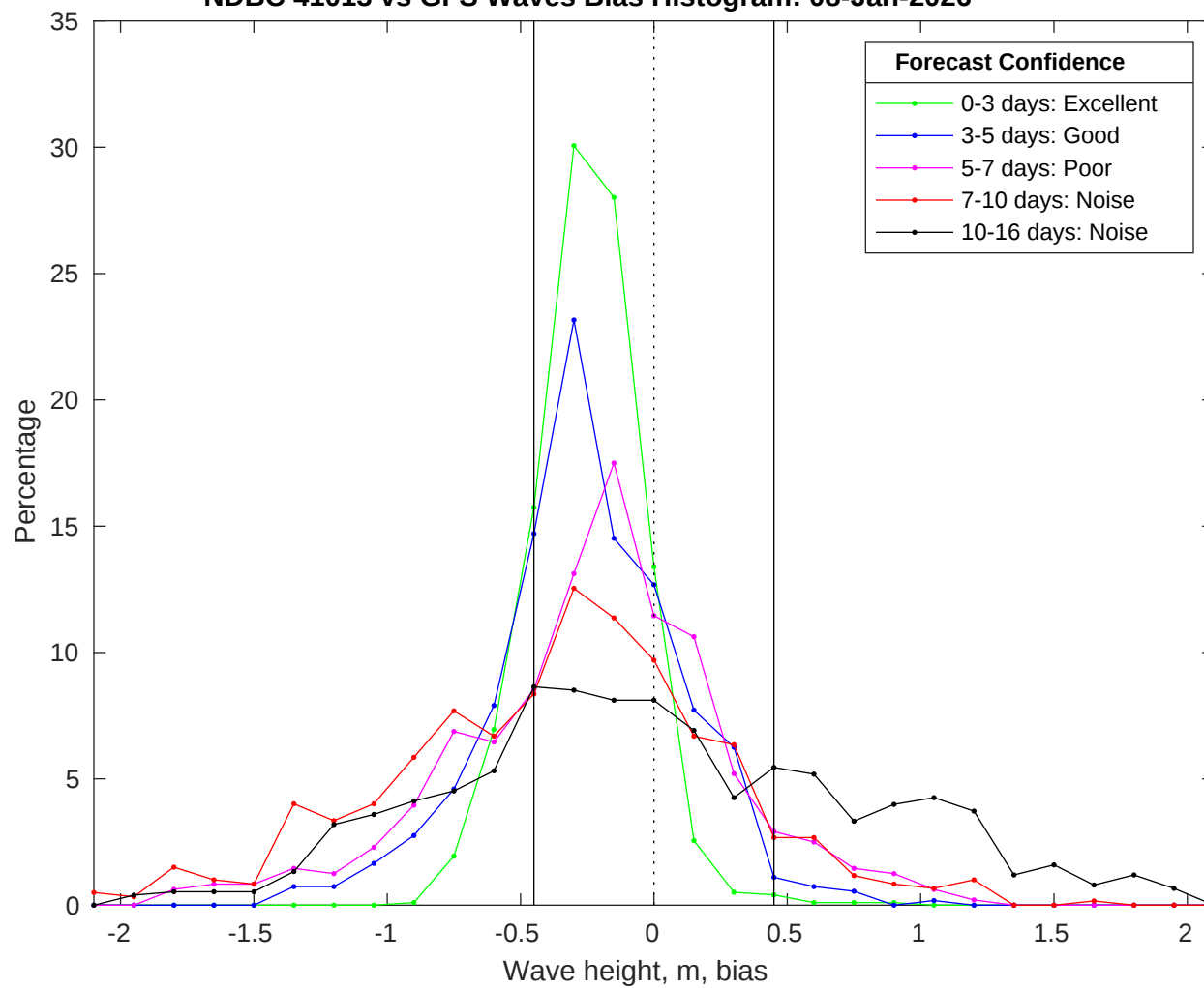
NDBC 41013 vs GFS Waves Bias Histogram: 08-Jan-2026
