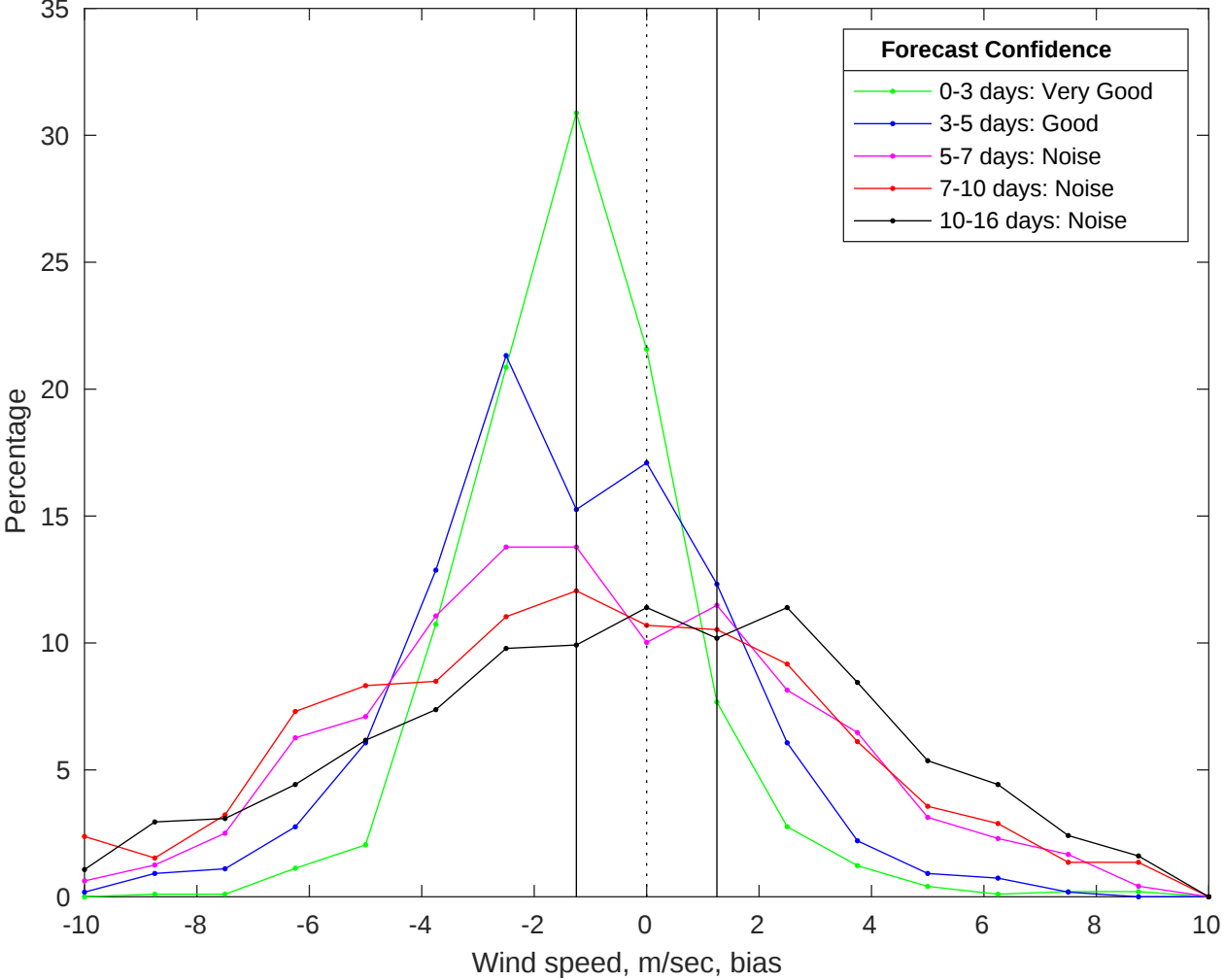
NDBC 41013 vs GFS Winds Bias Histogram: 08-Jan-2026
