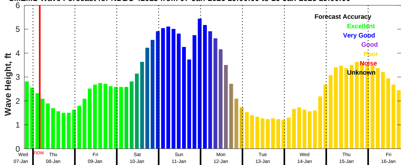
CMEMS Wave Forecast for NDBC 41013 from 07-Jan-2026 19:00:00 to 16-Jan-2026 19:00:00
