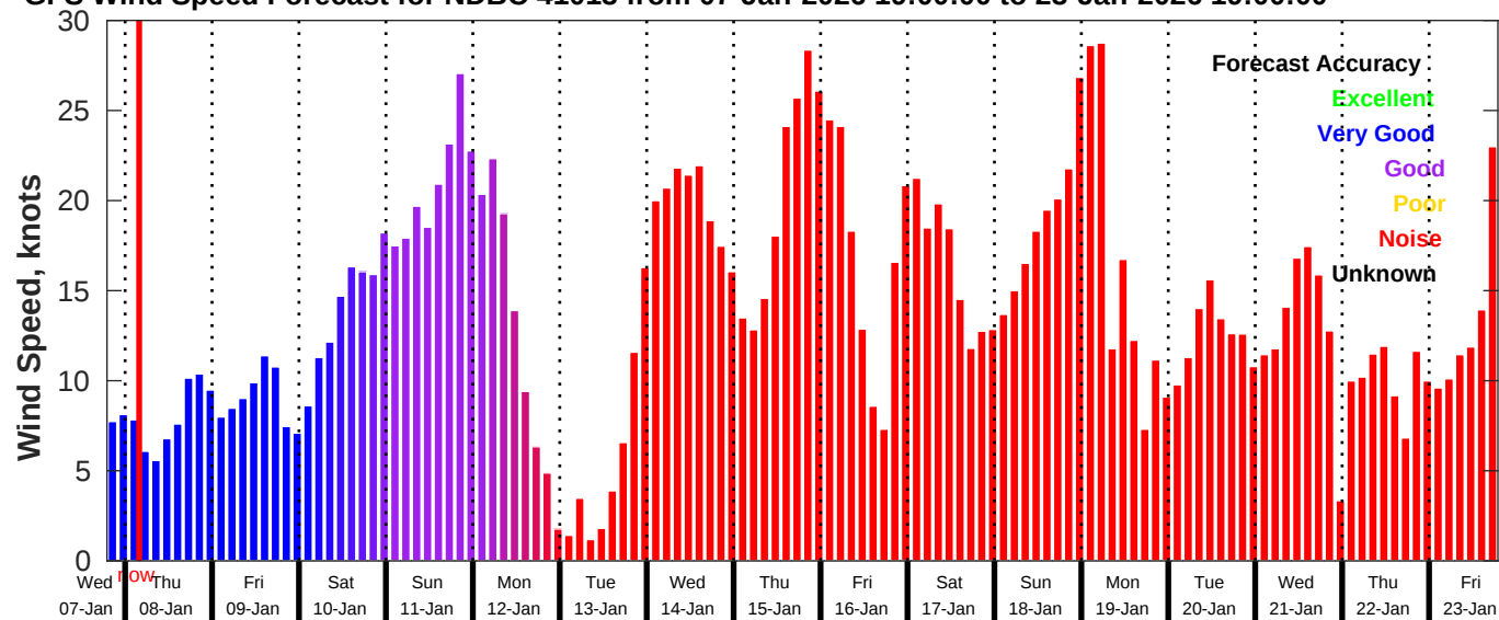
GFS Wind Speed Forecast for NDBC 41013 from 07-Jan-2026 19:00:00 to 23-Jan-2026 19:00:00
