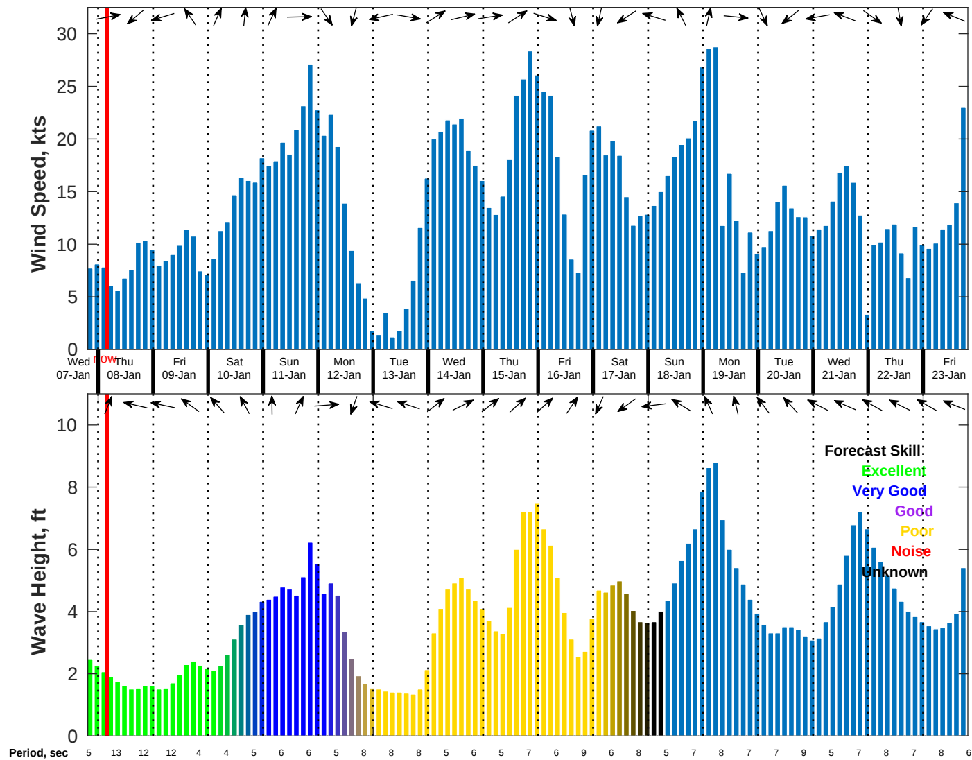
Wind & Wave Forecast for NDBC 41013 from 07-Jan-2026 19:00:00 to 23-Jan-2026 19:00:00
