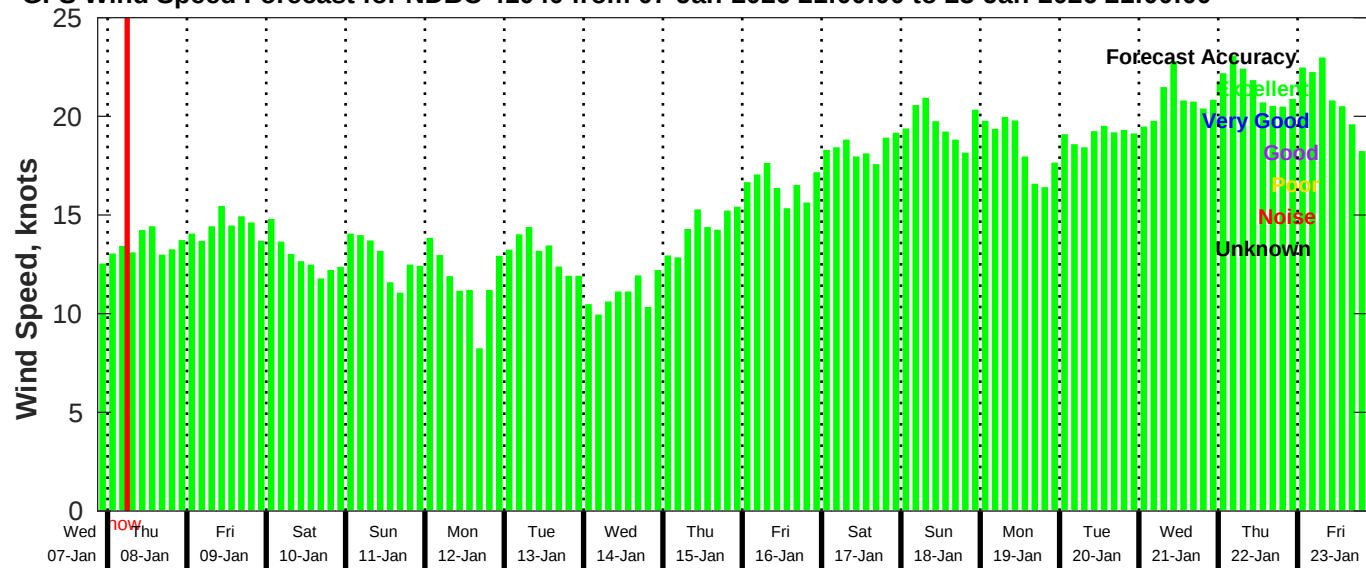
GFS Wind Speed Forecast for NDBC 41040 from 07-Jan-2026 21:00:00 to 23-Jan-2026 21:00:00
