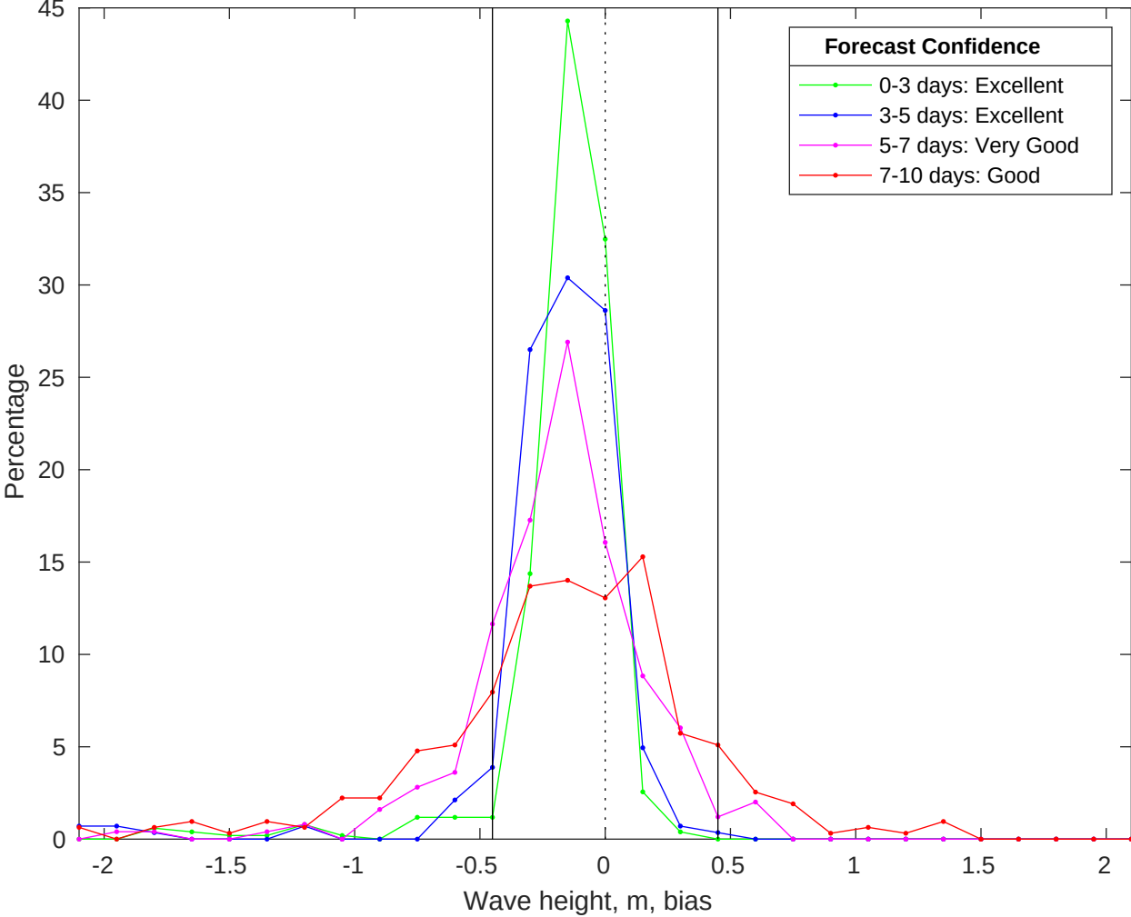
NDBC 42019 vs CMEMS Waves Bias Histogram: 08-Jan-2026
