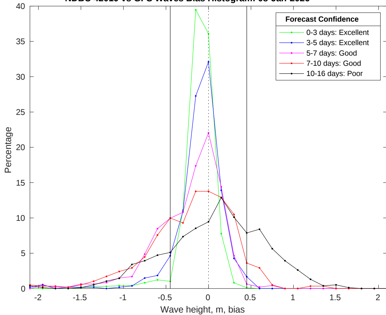
NDBC 42019 vs GFS Waves Bias Histogram: 08-Jan-2026
