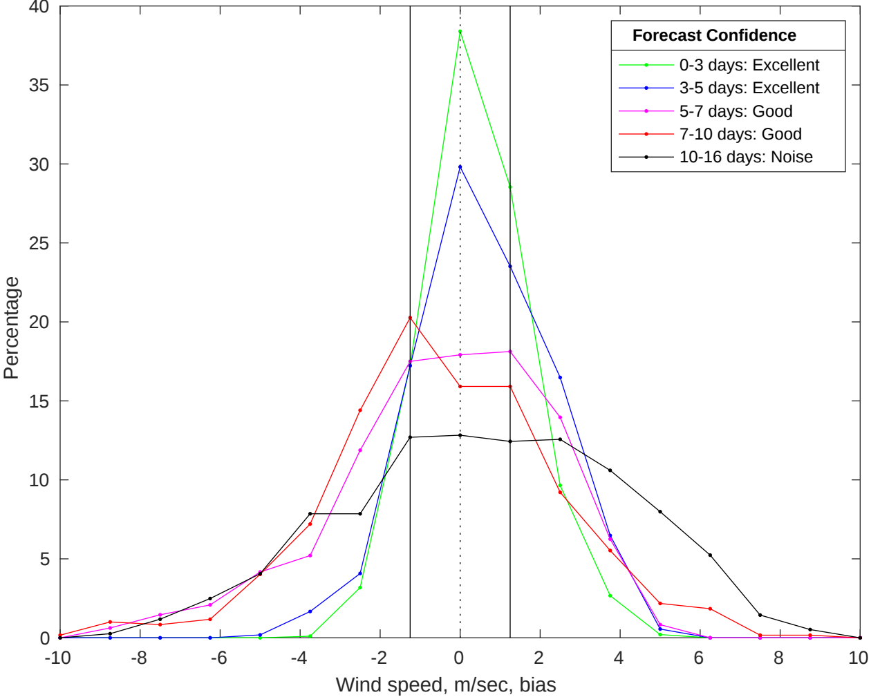
NDBC 42019 vs GFS Winds Bias Histogram: 08-Jan-2026
