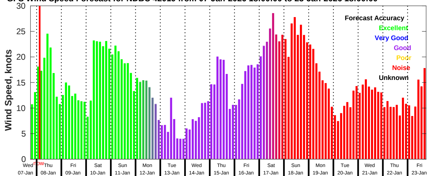
GFS Wind Speed Forecast for NDBC 42019 from 07-Jan-2026 18:00:00 to 23-Jan-2026 18:00:00
