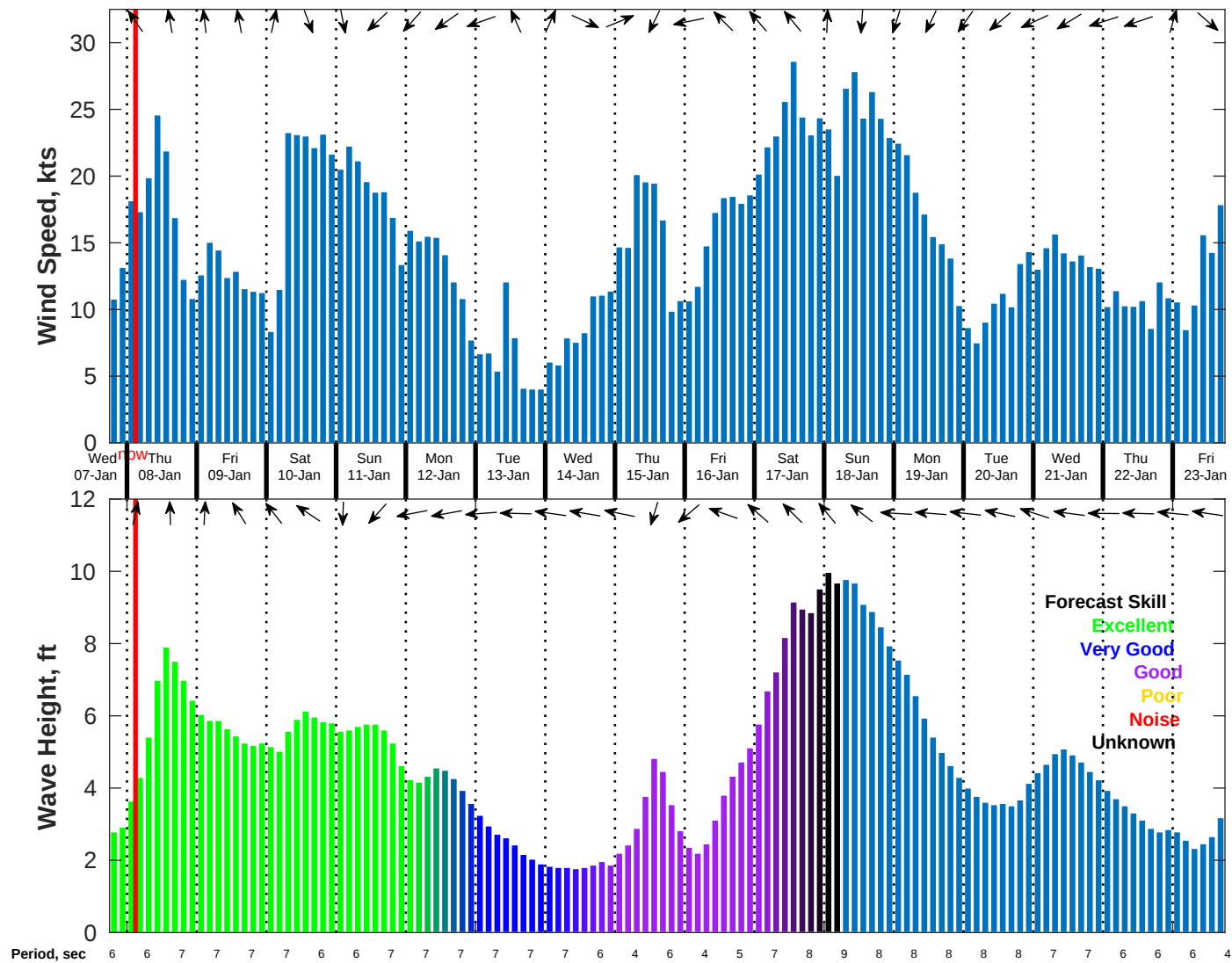
Wind & Wave Forecast for NDBC 42019 from 07-Jan-2026 18:00:00 to 23-Jan-2026 18:00:00
