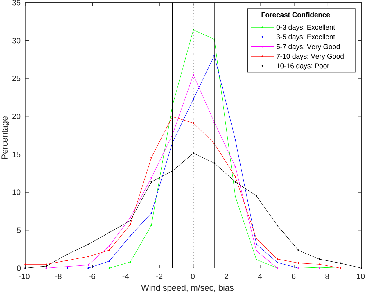
NDBC 42020 vs GFS Winds Bias Histogram: 08-Jan-2026
