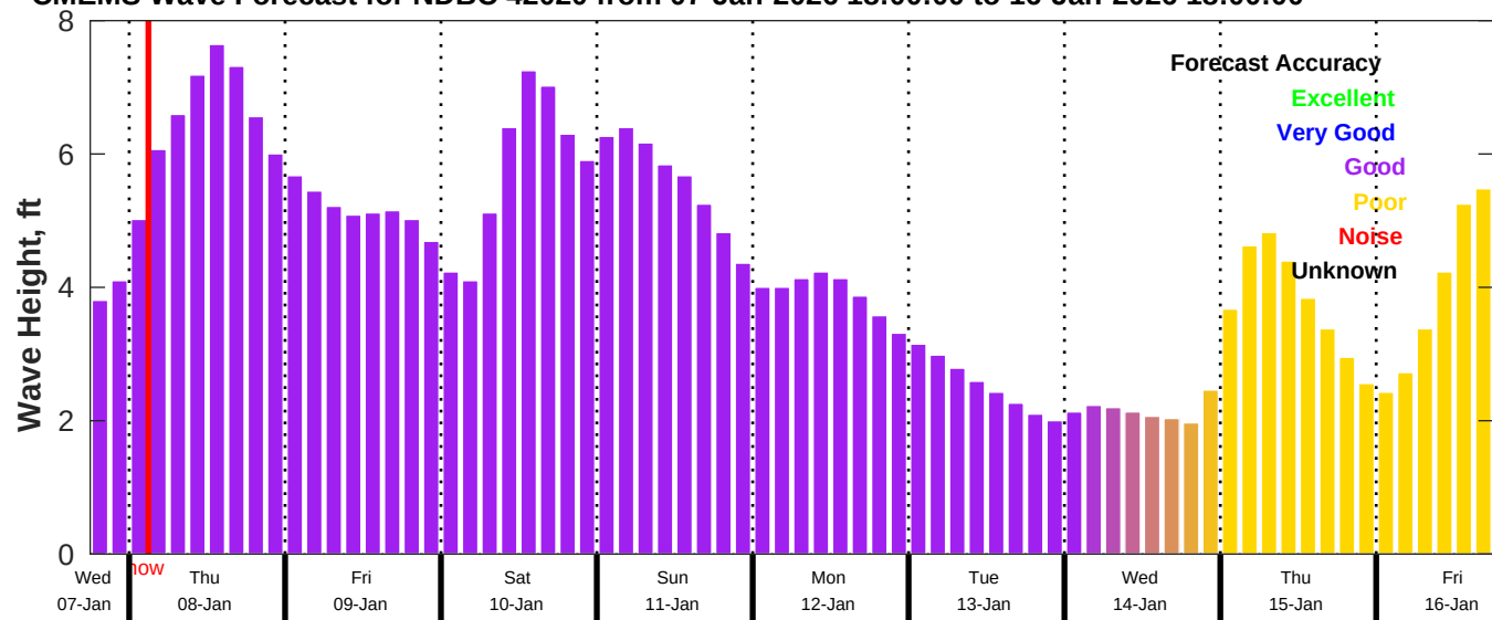
CMEMS Wave Forecast for NDBC 42020 from 07-Jan-2026 18:00:00 to 16-Jan-2026 18:00:00
