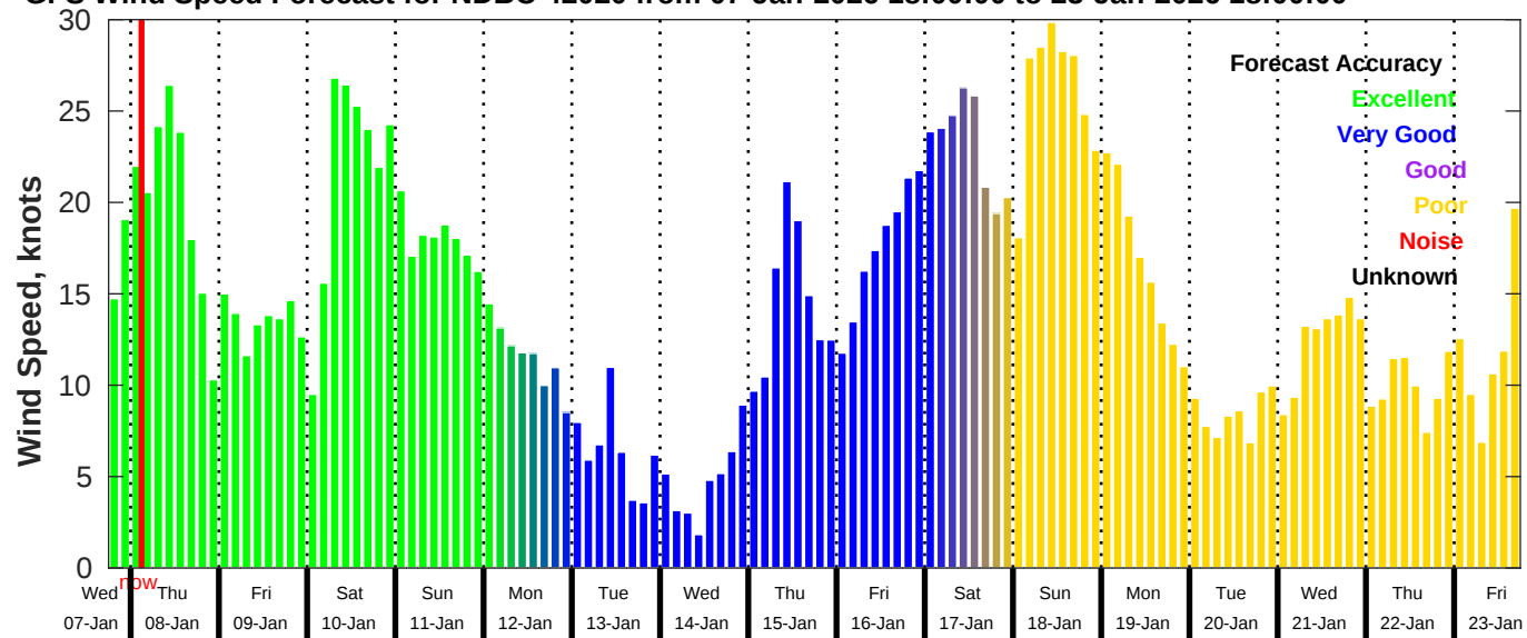
GFS Wind Speed Forecast for NDBC 42020 from 07-Jan-2026 18:00:00 to 23-Jan-2026 18:00:00
