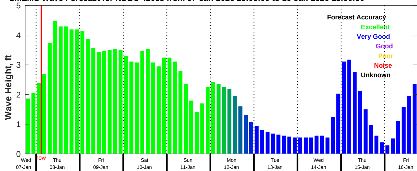
CMEMS Wave Forecast for NDBC 42035 from 07-Jan-2026 18:00:00 to 16-Jan-2026 18:00:00
