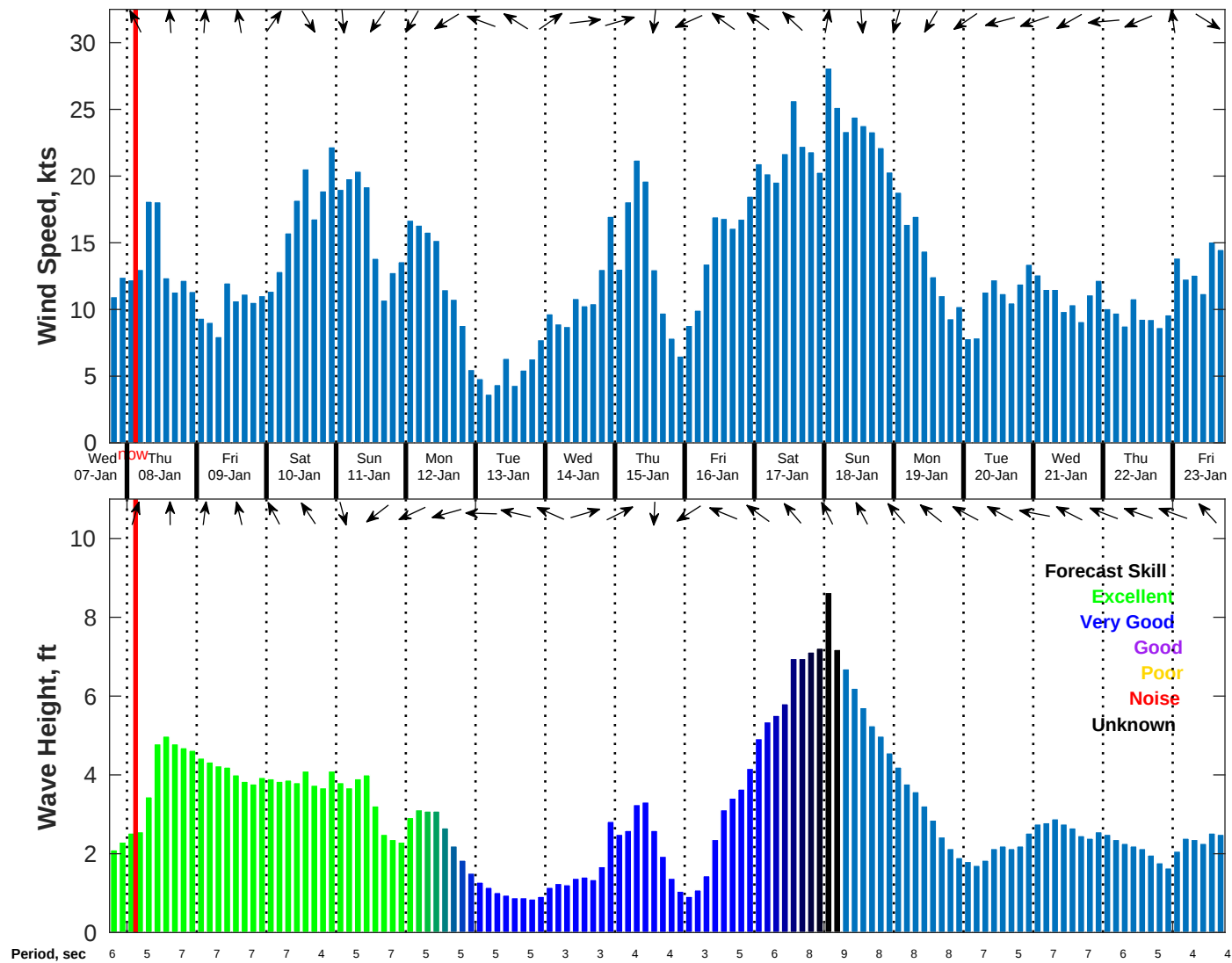
Wind & Wave Forecast for NDBC 42035 from 07-Jan-2026 18:00:00 to 23-Jan-2026 18:00:00
