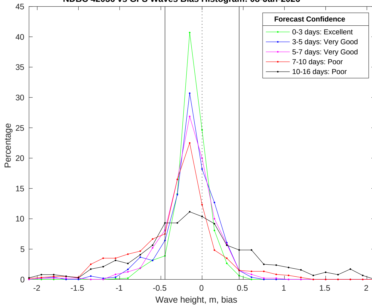
NDBC 42036 vs GFS Waves Bias Histogram: 08-Jan-2026
