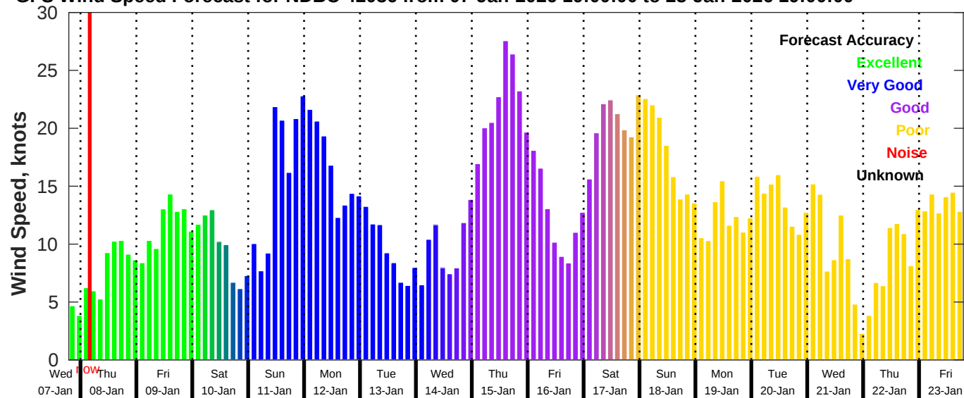
GFS Wind Speed Forecast for NDBC 42036 from 07-Jan-2026 19:00:00 to 23-Jan-2026 19:00:00
