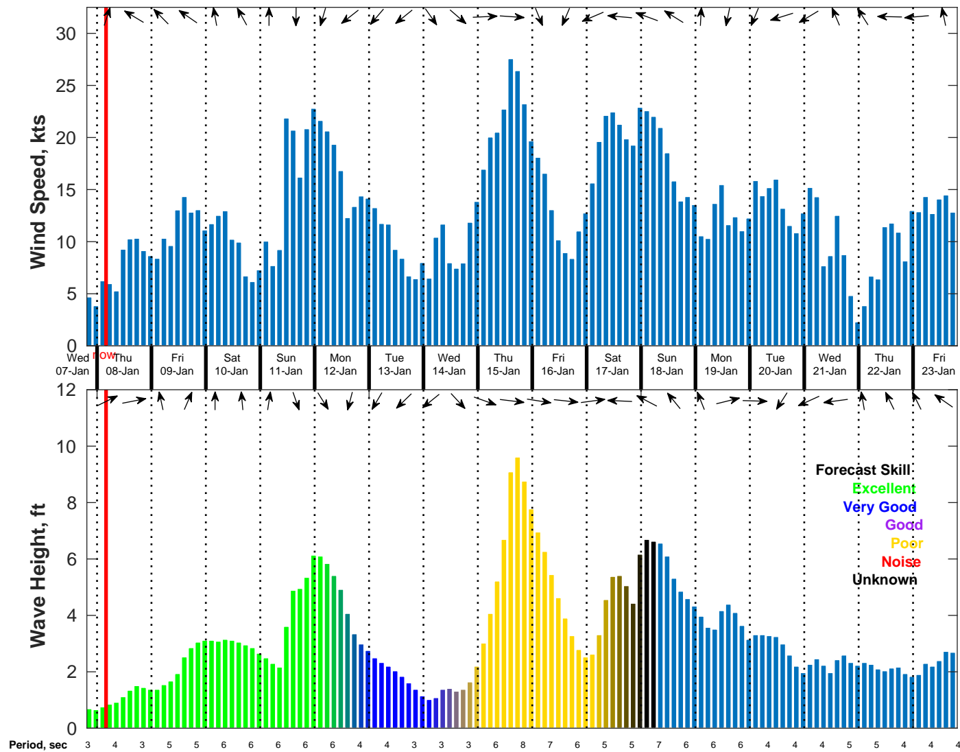
Wind & Wave Forecast for NDBC 42036 from 07-Jan-2026 19:00:00 to 23-Jan-2026 19:00:00
