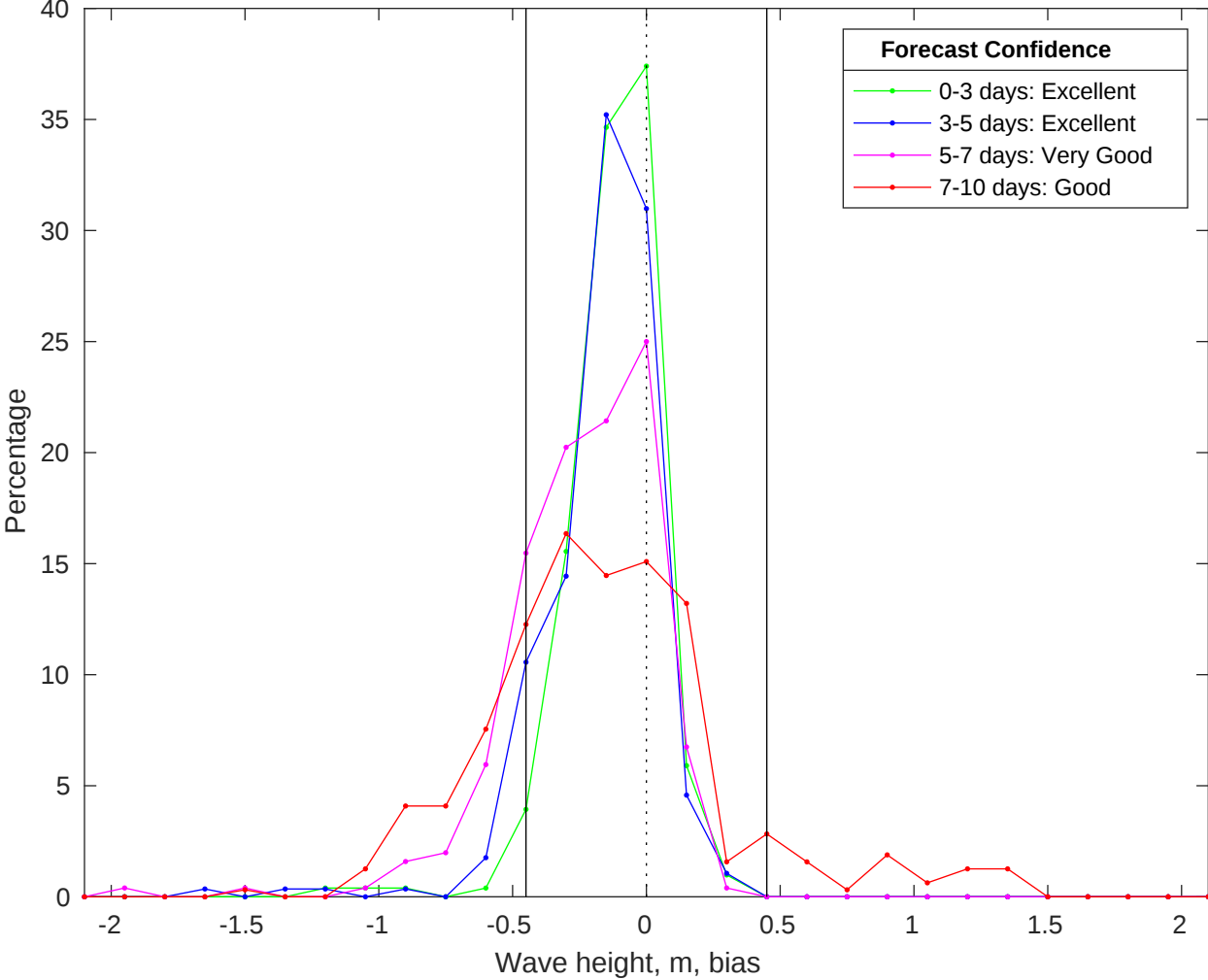
NDBC 42040 vs CMEMS Waves Bias Histogram: 08-Jan-2026
