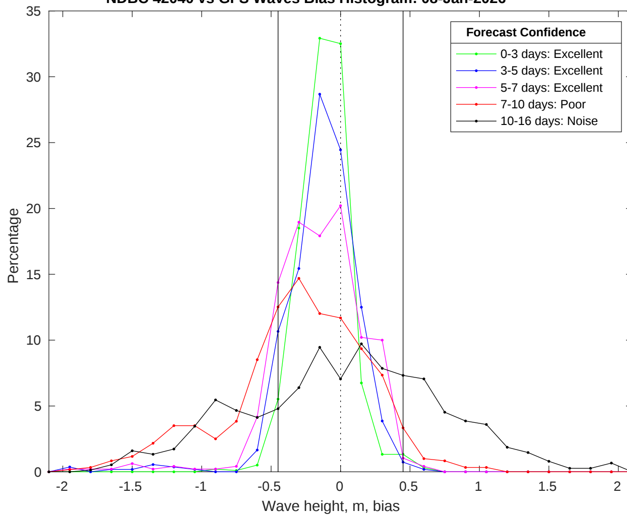
NDBC 42040 vs GFS Waves Bias Histogram: 08-Jan-2026
