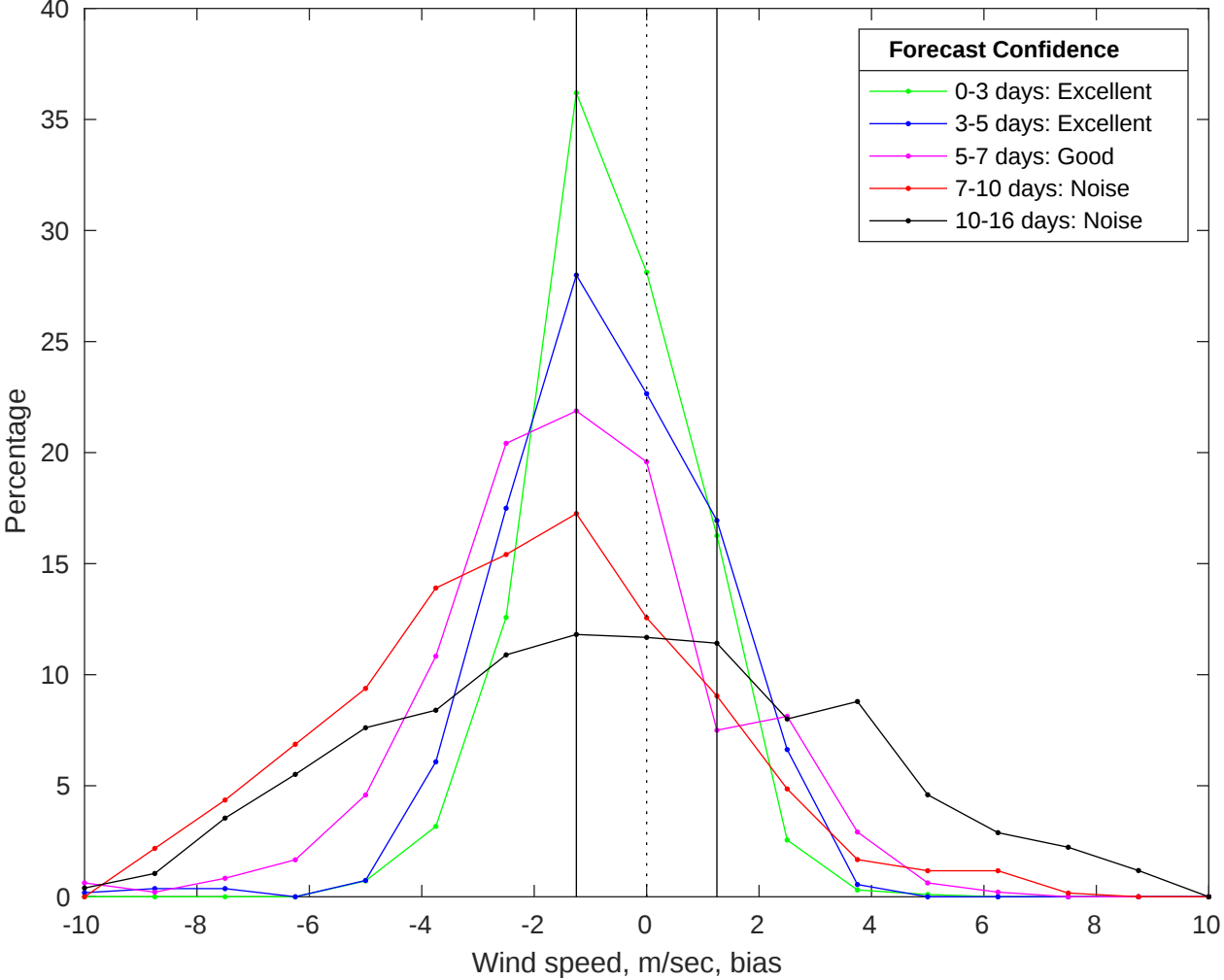
NDBC 42040 vs GFS Winds Bias Histogram: 08-Jan-2026
