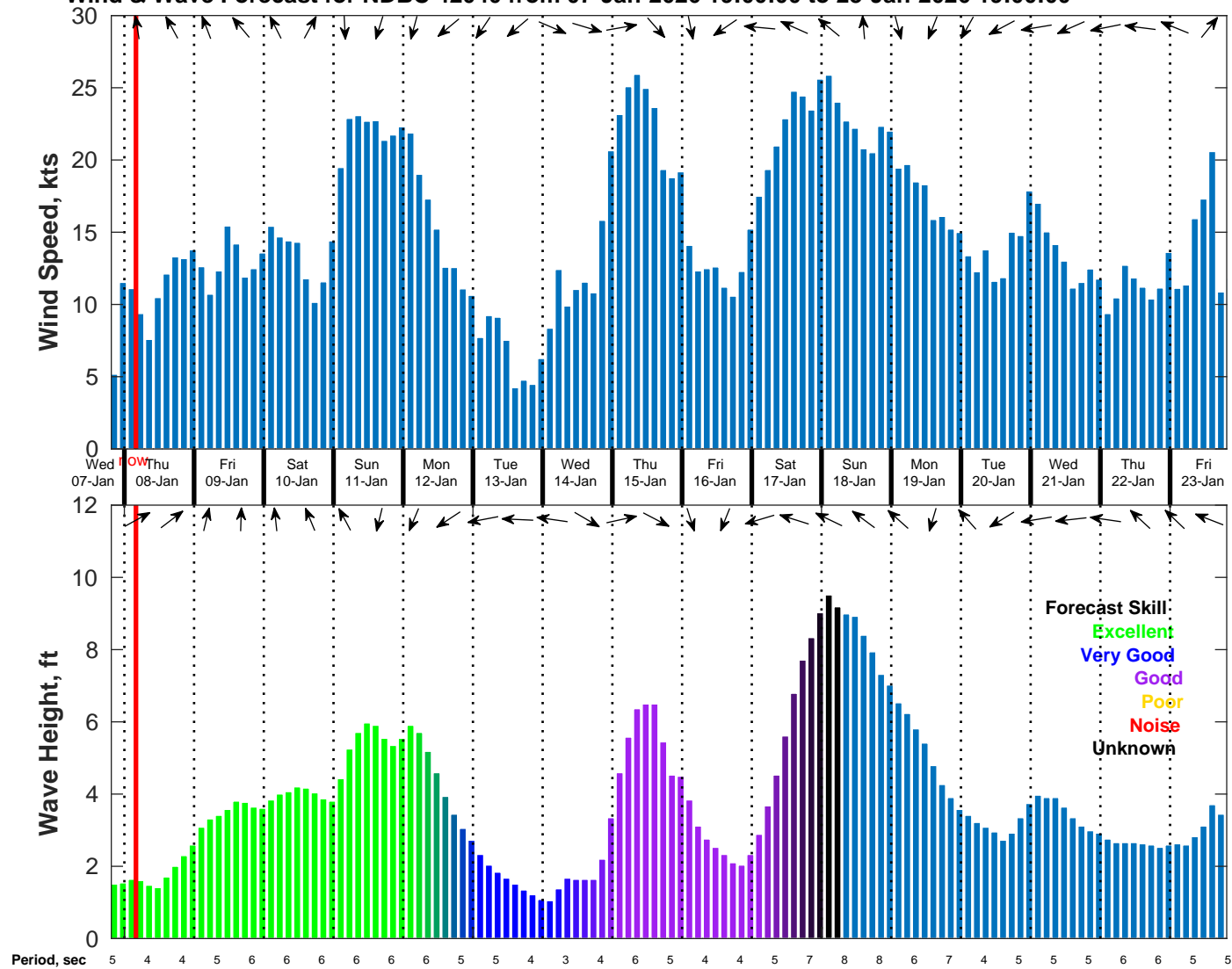
Wind & Wave Forecast for NDBC 42040 from 07-Jan-2026 19:00:00 to 23-Jan-2026 19:00:00
