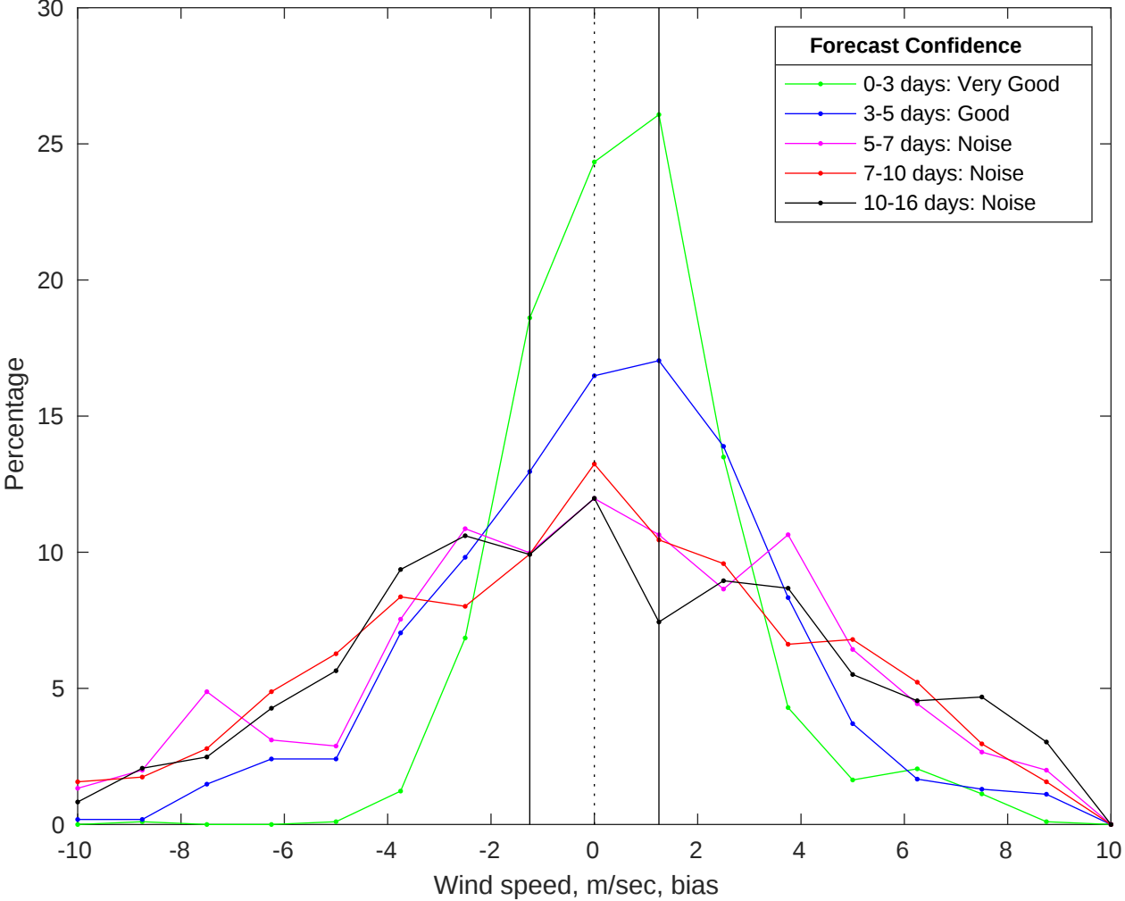
NDBC 44008 vs GFS Winds Bias Histogram: 08-Jan-2026
