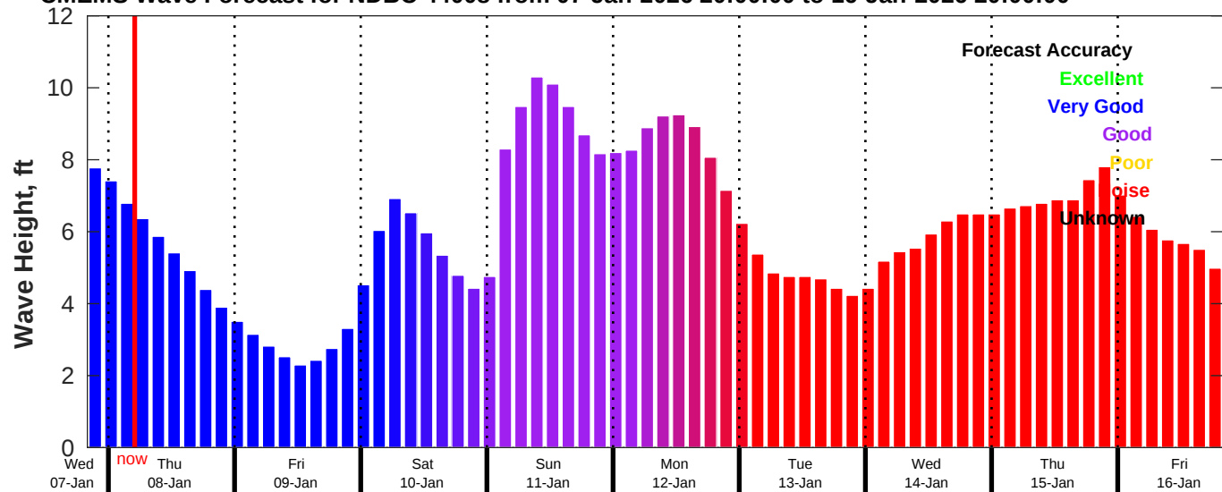
CMEMS Wave Forecast for NDBC 44008 from 07-Jan-2026 20:00:00 to 16-Jan-2026 20:00:00
