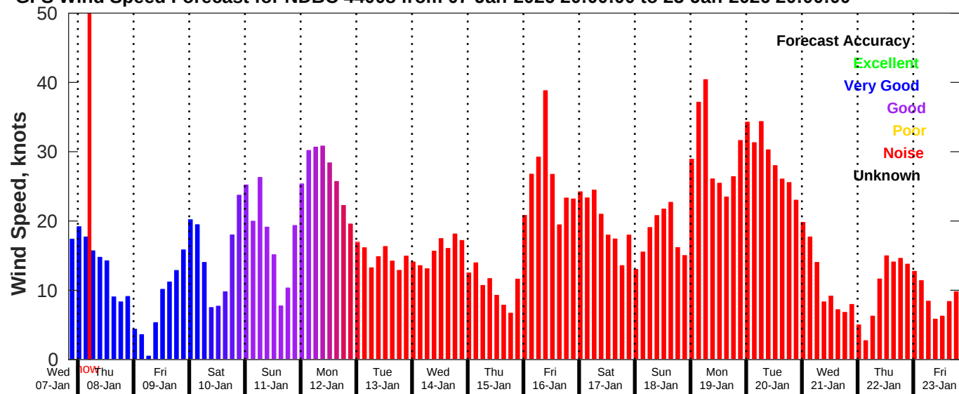
GFS Wind Speed Forecast for NDBC 44008 from 07-Jan-2026 20:00:00 to 23-Jan-2026 20:00:00
