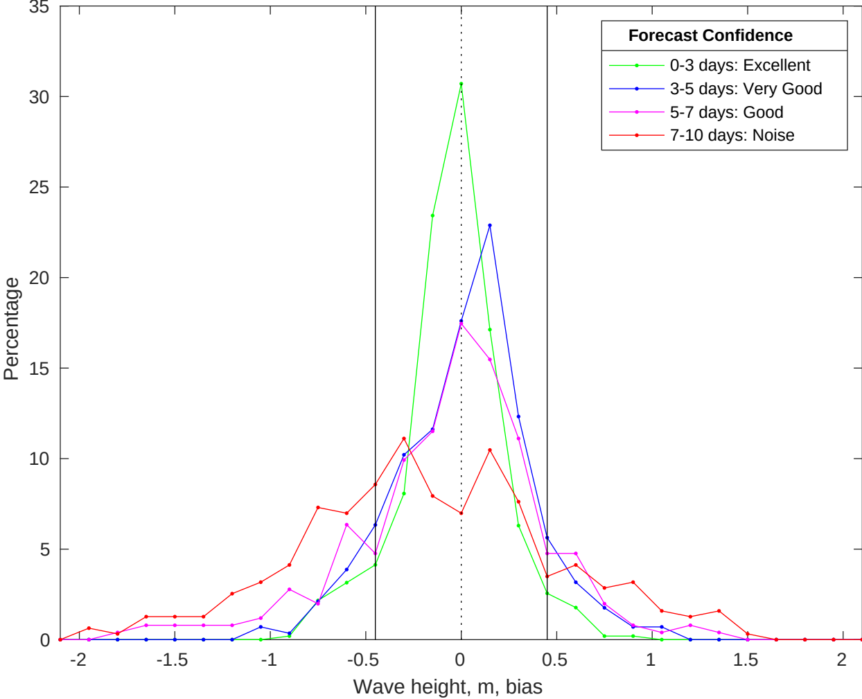
NDBC 46011 vs CMEMS Waves Bias Histogram: 08-Jan-2026
