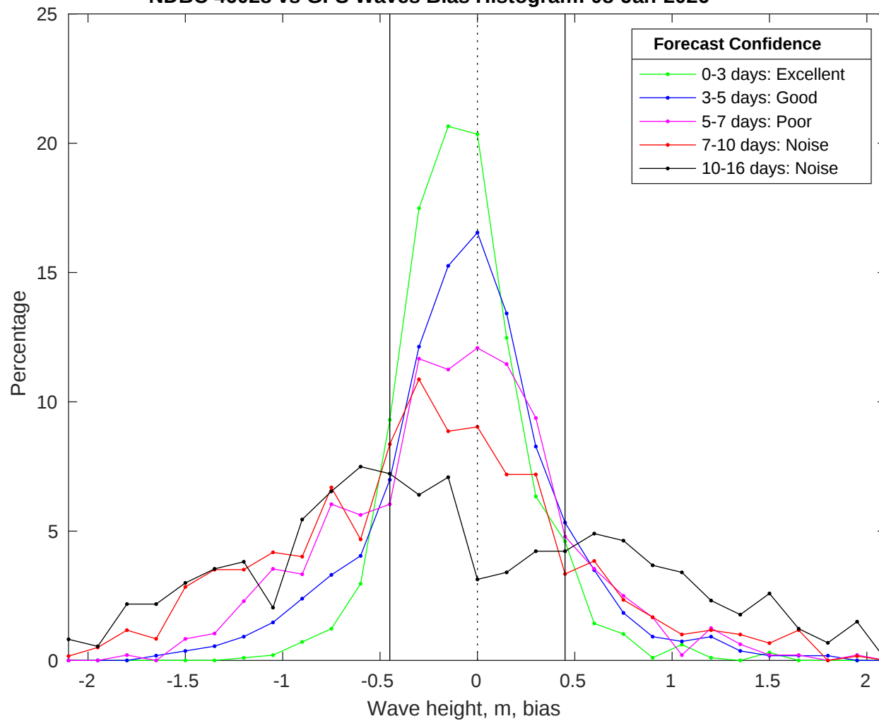
NDBC 46028 vs GFS Waves Bias Histogram: 08-Jan-2026
