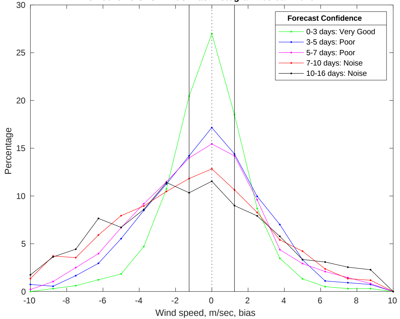
NDBC 46028 vs GFS Winds Bias Histogram: 08-Jan-2026
