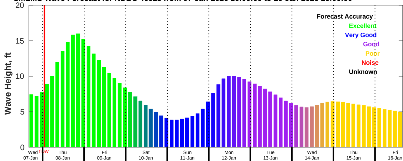
CMEMS Wave Forecast for NDBC 46028 from 07-Jan-2026 16:00:00 to 16-Jan-2026 16:00:00
