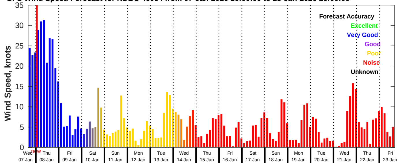
GFS Wind Speed Forecast for NDBC 46054 from 07-Jan-2026 16:00:00 to 23-Jan-2026 16:00:00
