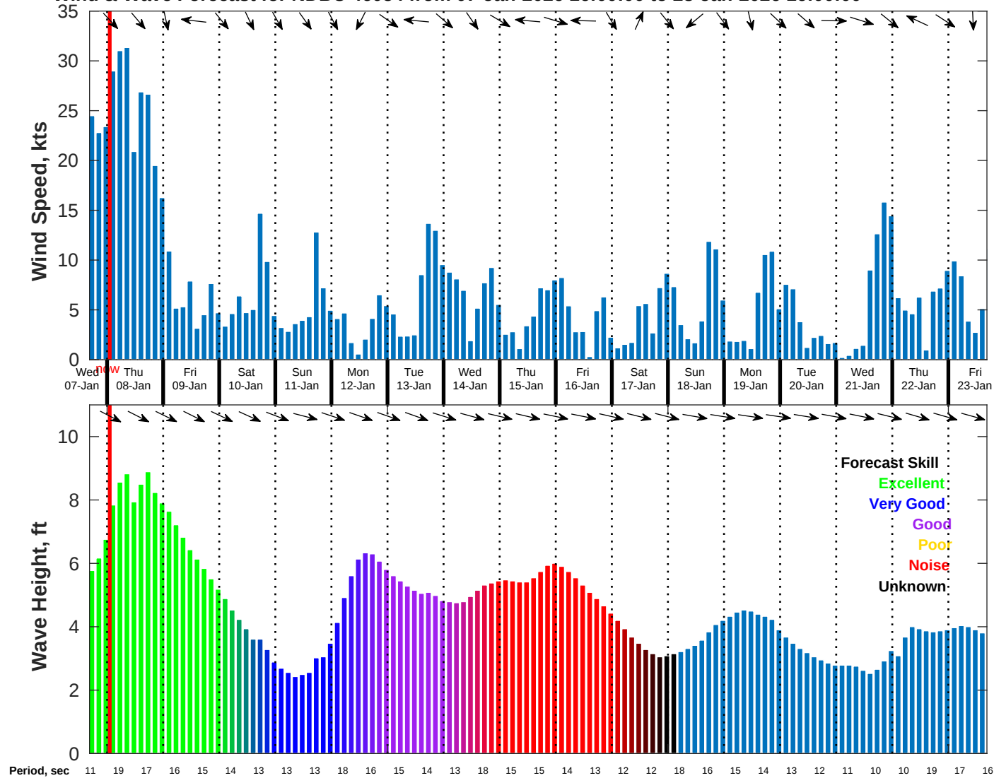
Wind & Wave Forecast for NDBC 46054 from 07-Jan-2026 16:00:00 to 23-Jan-2026 16:00:00
