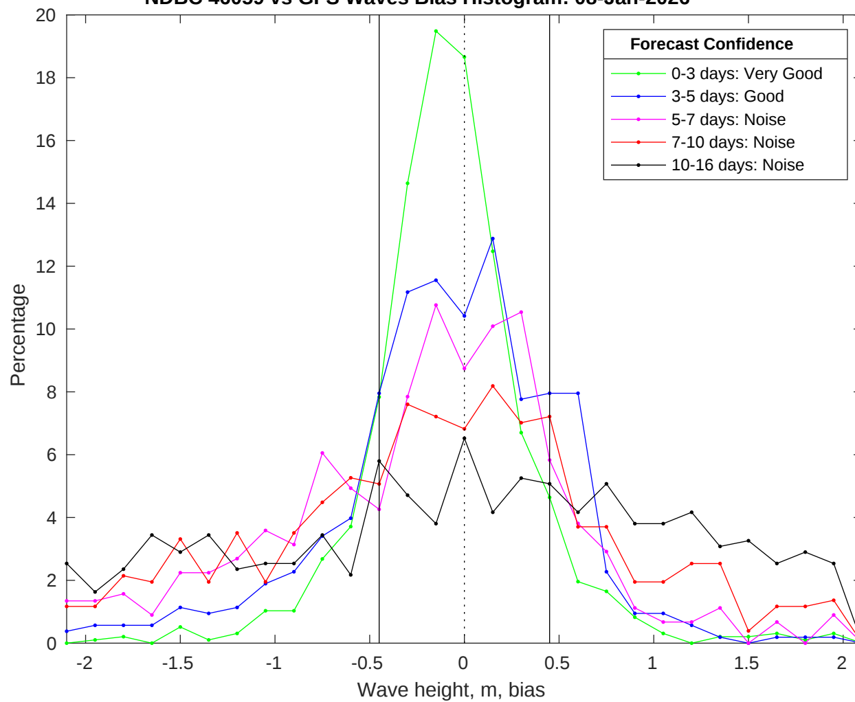
NDBC 46059 vs GFS Waves Bias Histogram: 08-Jan-2026
